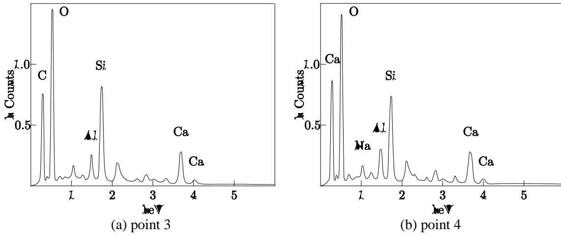
Fig. 7.10 EDS spectrum of matrix
