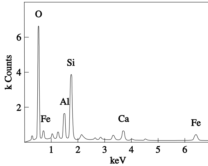
Fig. E- 2 DEX spectrum – point 1
