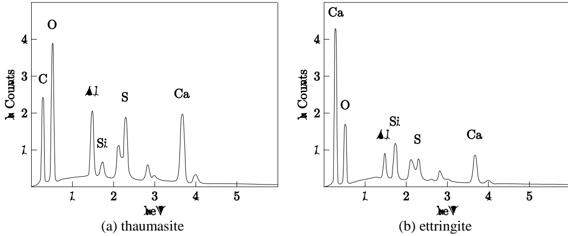
Fig. 7.16 EDX result for the minerals in void A
