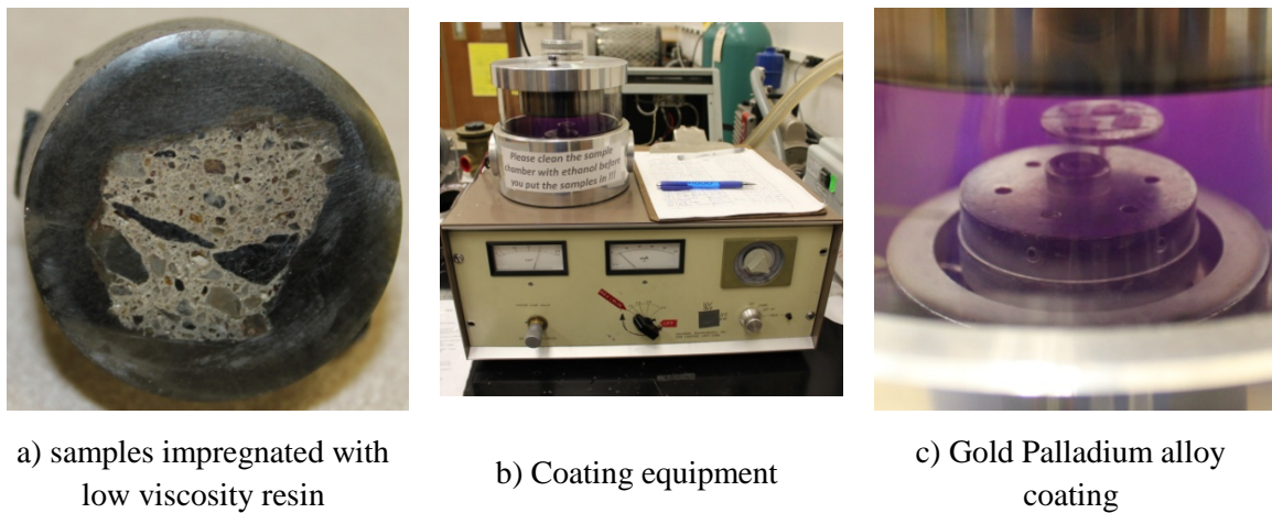
Fig. 5.10 SEM sample preparation
