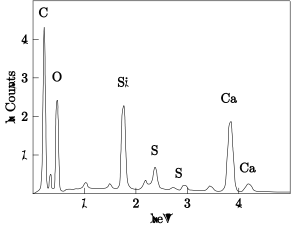
Fig. F- 4 EDS spectrum of point 3 matrix
